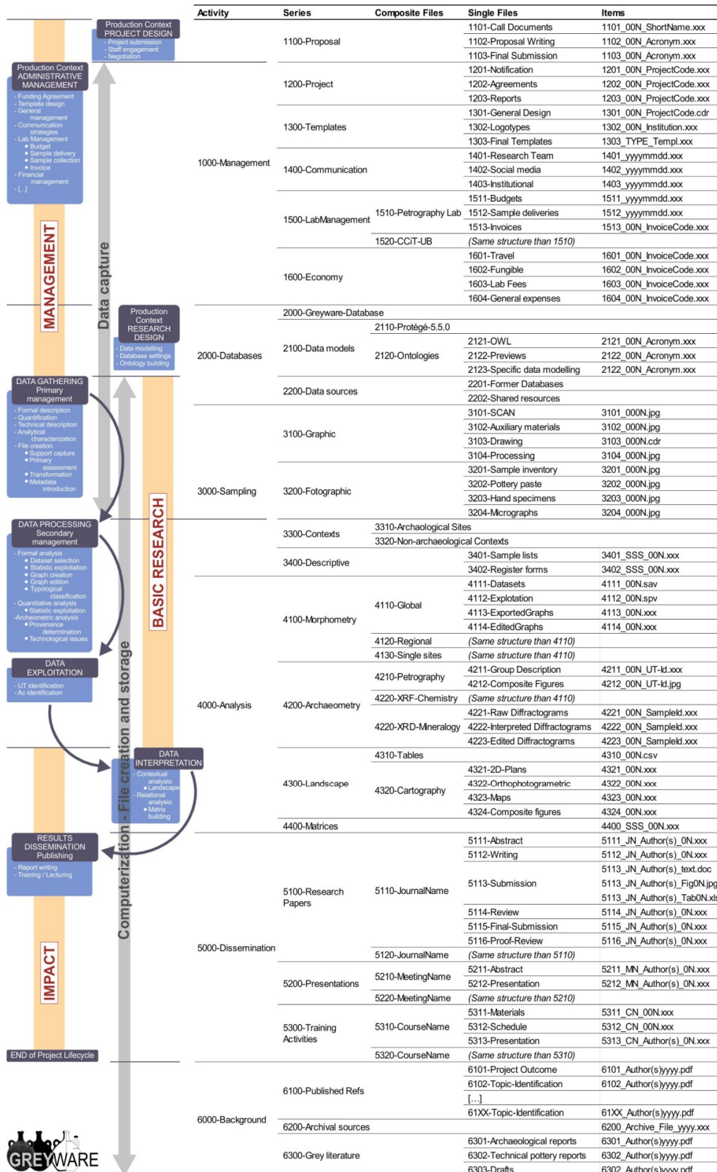
Figure 3. Classification chart of processes, series and files.
