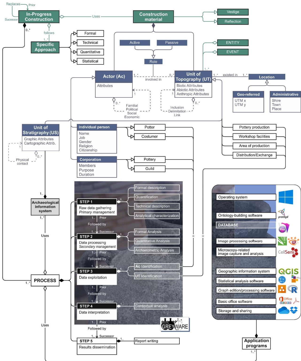
Figure 4. UML diagram of GREYWARE’s overview and components. Classes described by the HORAI UT/Ac data model are represented in blue. Their relation with top-level entity-event ontologies [11,35] are highlighted in green. Categories defined in pottery studies (and thus in domain or task ontologies) included in the GREYWARE data-modelling are represented in black and white. The central area shaded by the project’s interface identifies the processes developed in the classification chart shown in Figure 2 and the application programs used to perform research tasks. Process components included in the GREYWARE database are shaded in white.
