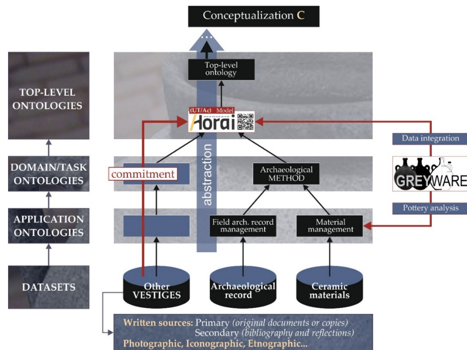
Figure 1. Graphic representation of the GREYWARE ontological commitment to the HORAI UT/Ac model as a top-level ontology.
