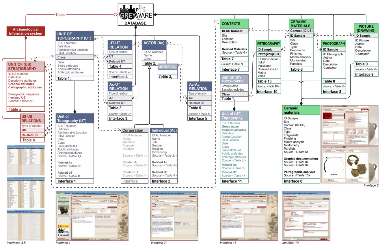
Figure 6. UML diagram of the GREYWARE database table-structure and components. The system commits a domain (pottery analysis) ontology and a top-level (HORAI UT/Ac) ontology whose categories are represented in green and blue shading, respectively.
